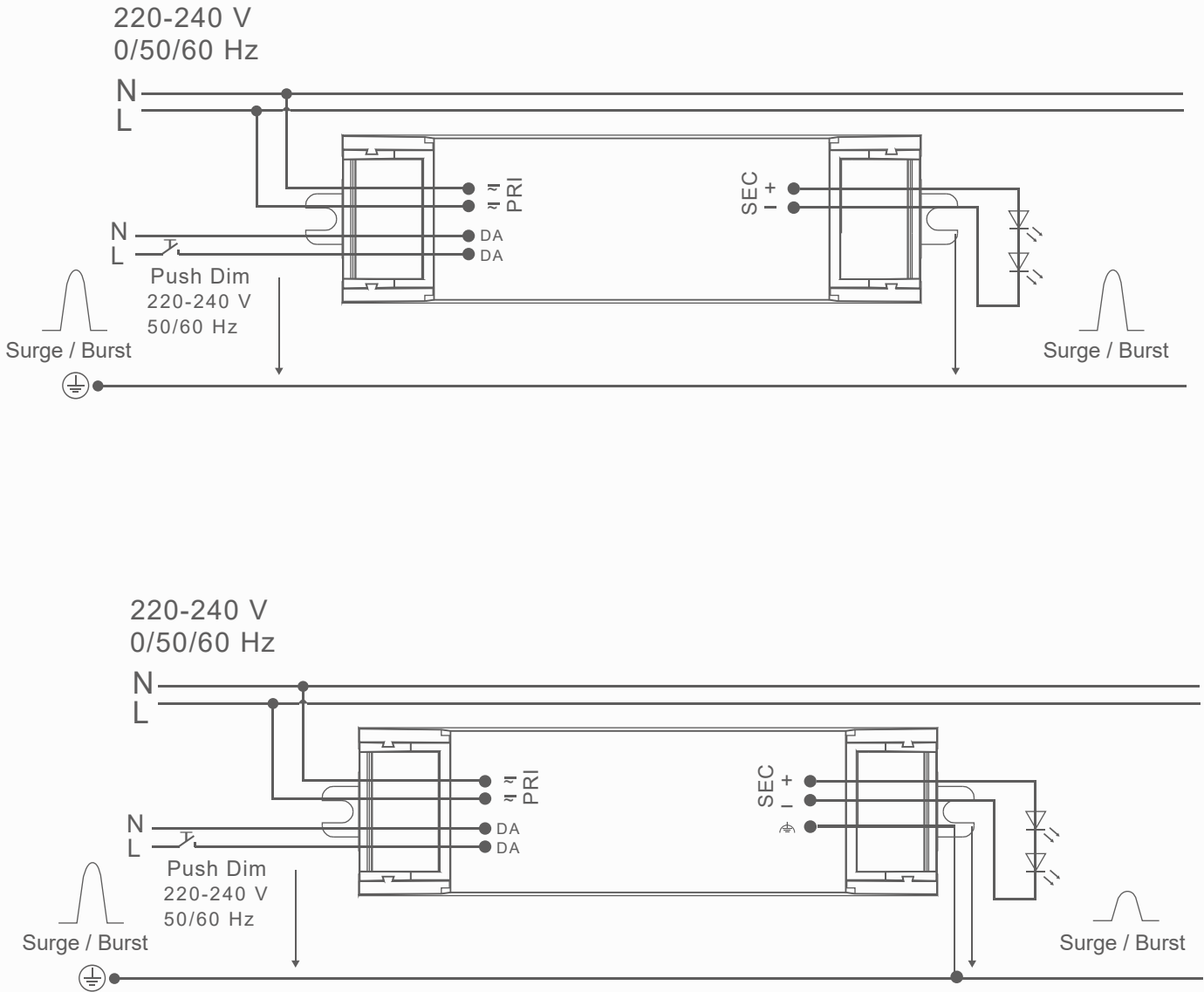
Fig.B:Push Dimming
