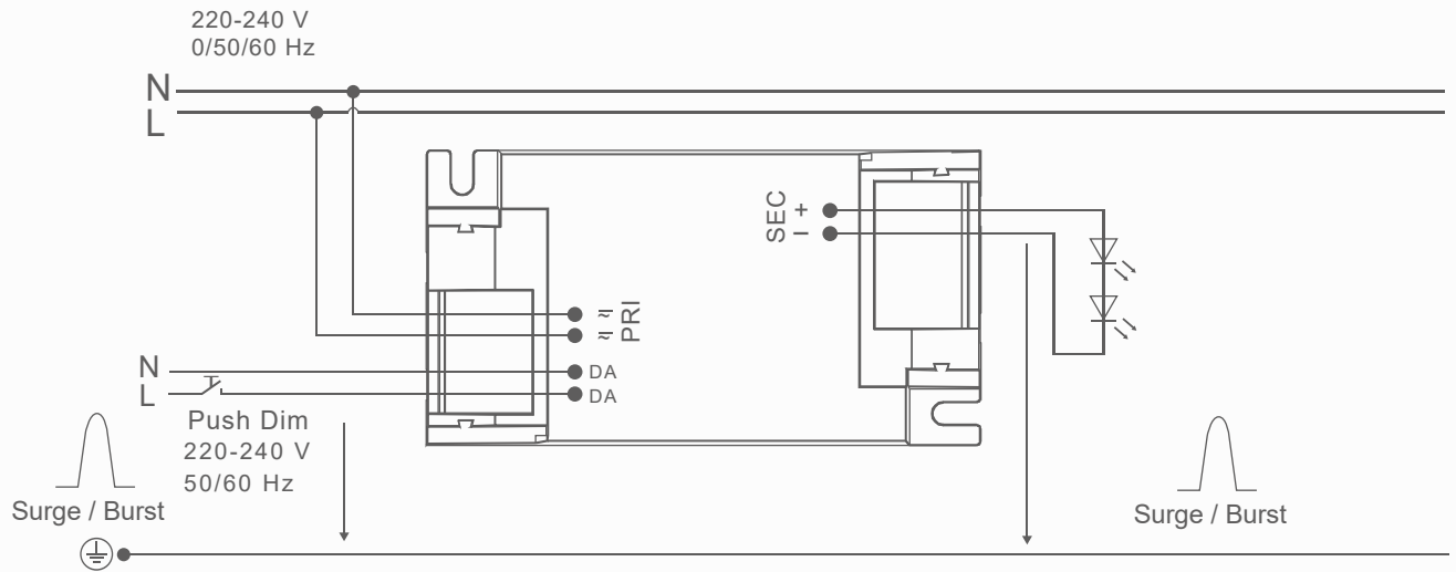
Fig.A: PushDimming
